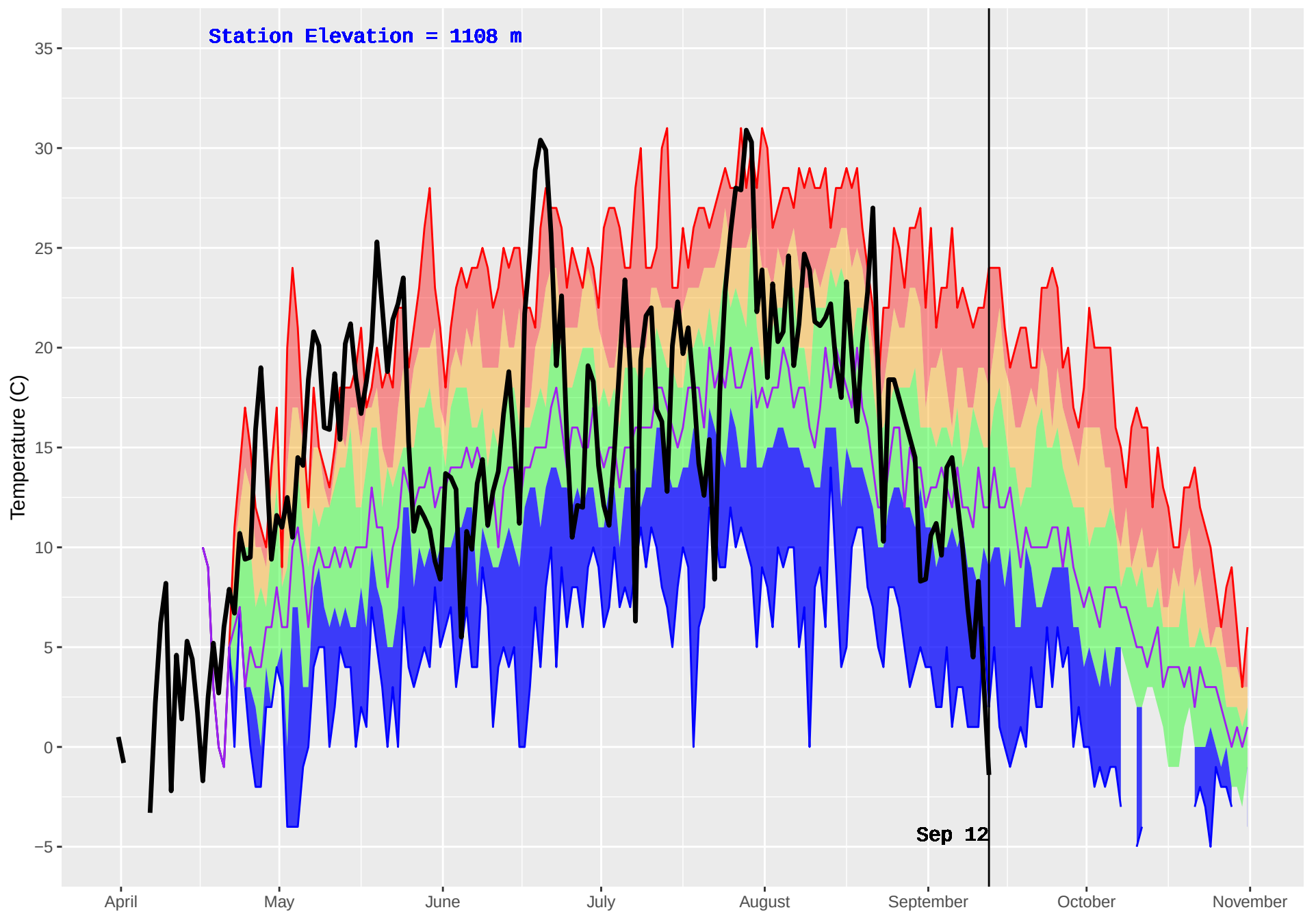
NABESHE (151) : Historical (1987–2016) and Current (2018) Daily Temperature
