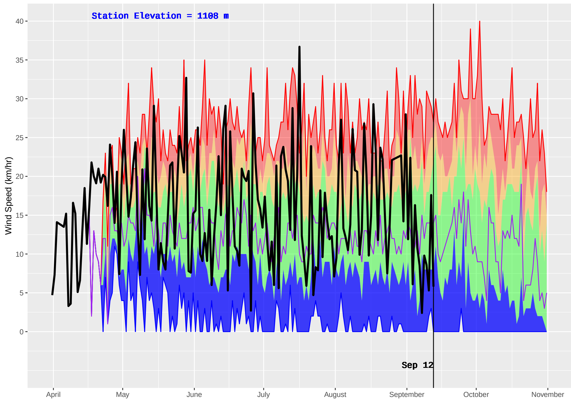
NABESHE (151) : Historical (1987–2016) and Current (2018) Daily Wind Speed
