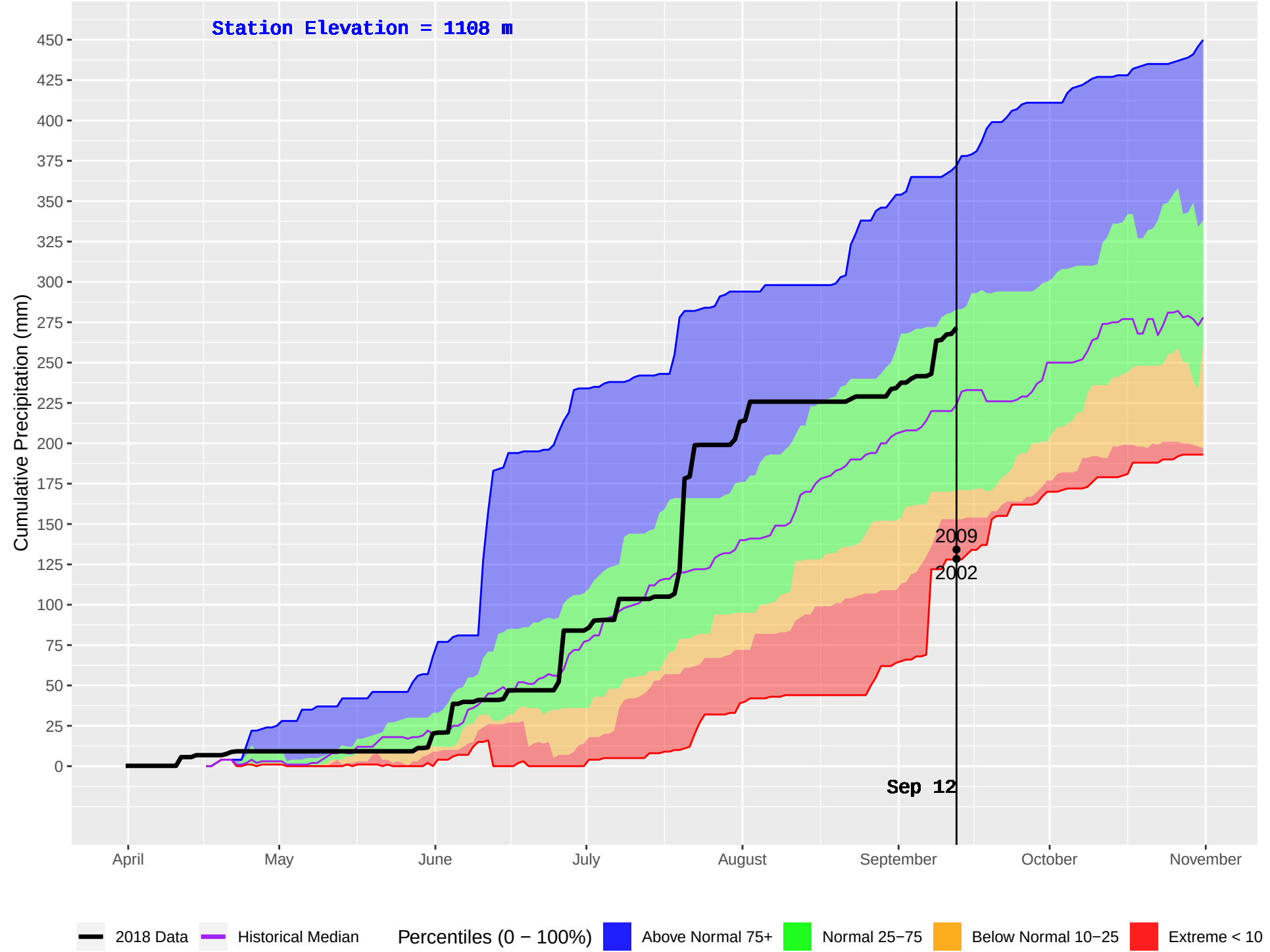
NABESHE (151) : Historical (1987–2016) and Current (2018) Daily Cumulative Precipitation
