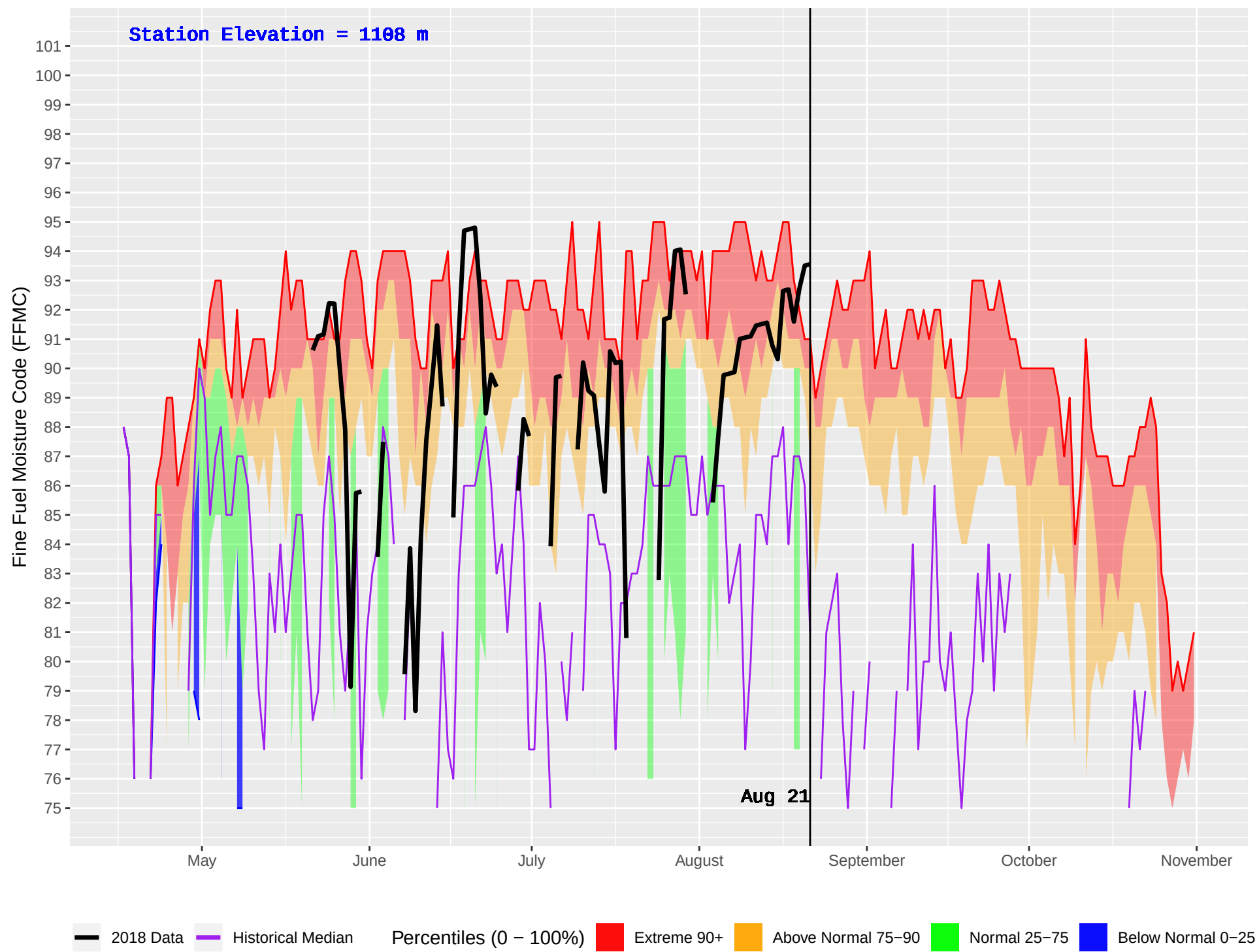
NABESHE (151) : Historical (1987–2016) and Current (2018) Daily Fine Fuel Moisture Code (FFMC)
