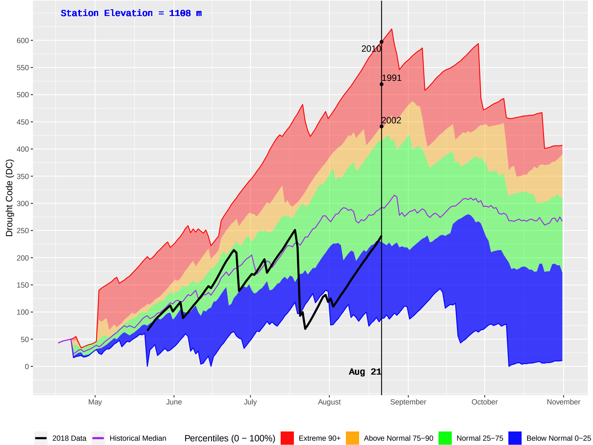
NABESHE (151) : Historical (1987–2016) and Current (2018) Daily Drought Code (DC)
