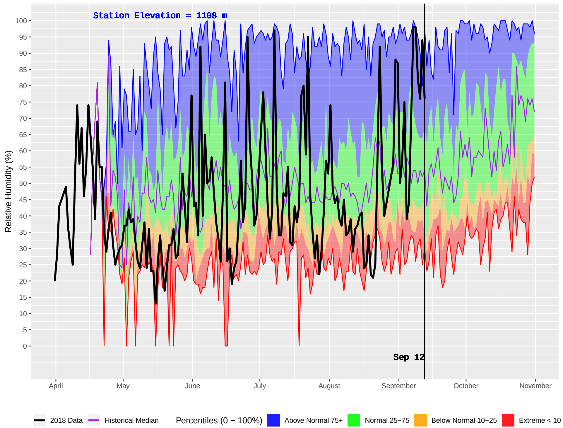
NABESHE (151) : Historical (1987–2016) and Current (2018) Daily Relative Humidity
