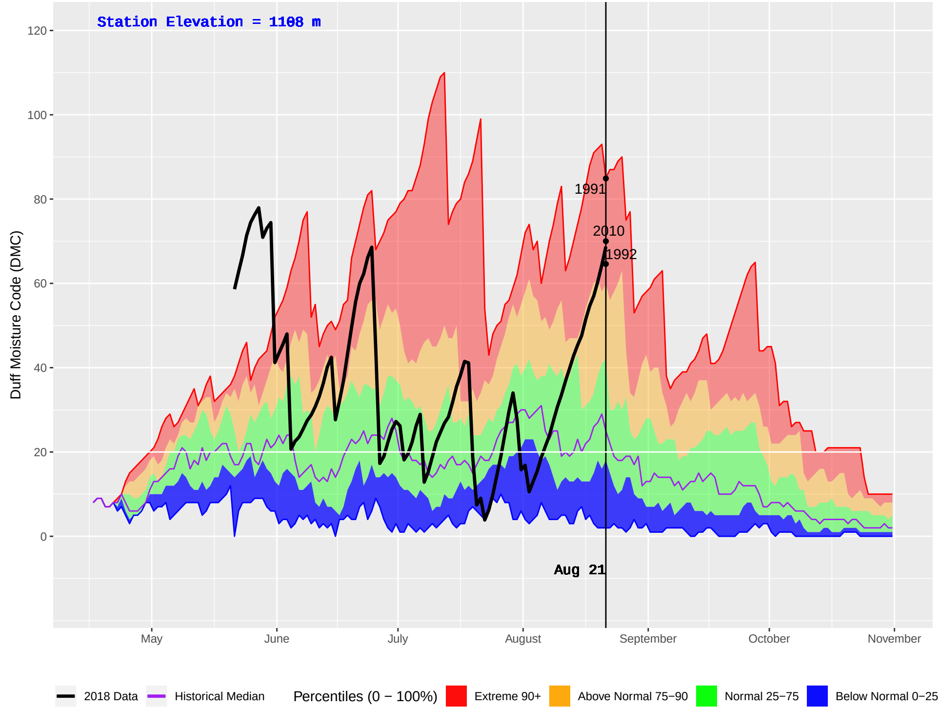
NABESHE (151) : Historical (1987–2016) and Current (2018) Daily Duff Moisture Code (DMC)
