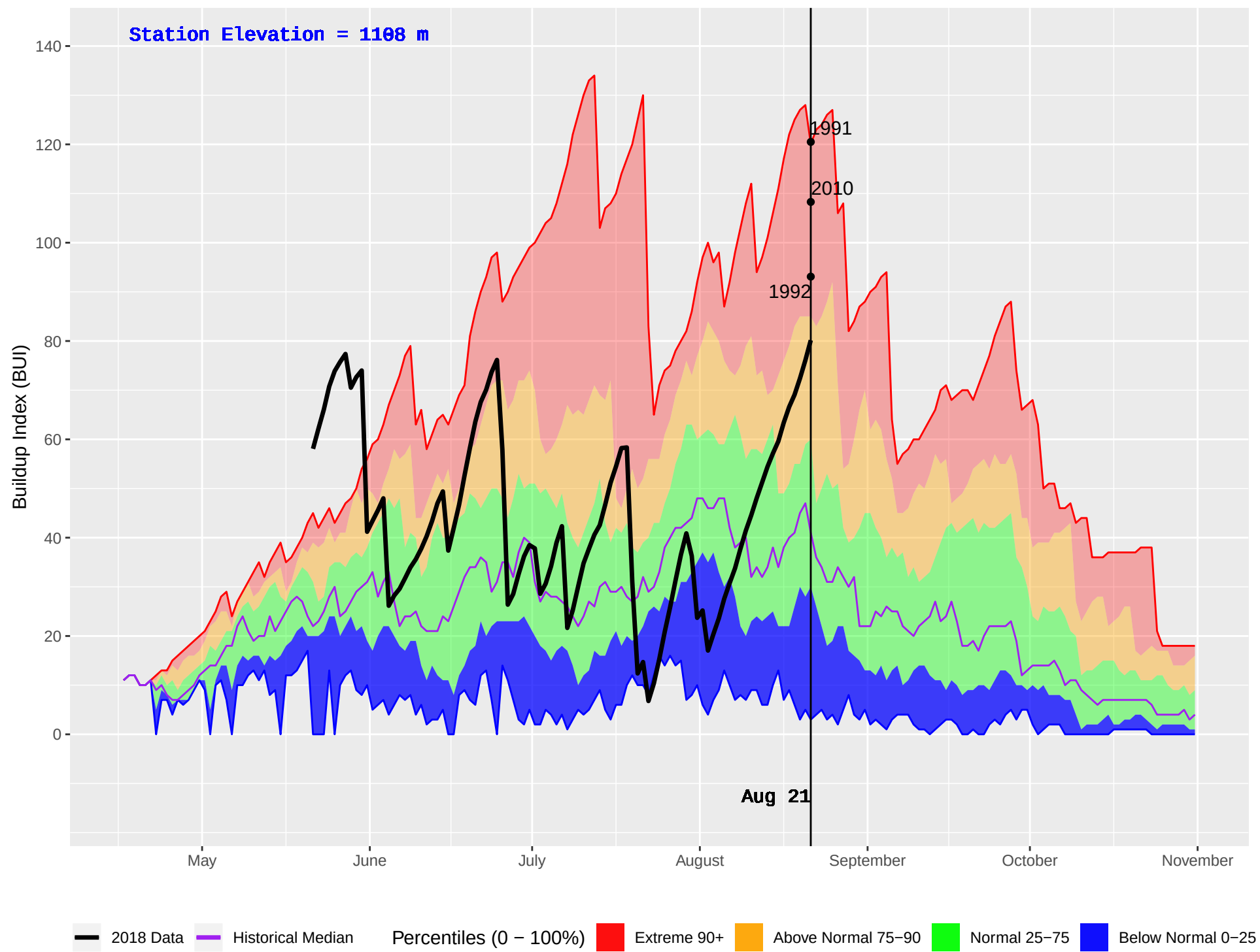
NABESHE (151) : Historical (1987–2016) and Current (2018) Daily Buildup Index (BUI)
